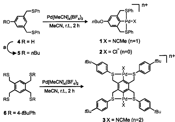
Scheme 2. Synthesis of SCS Pd II pincer complexes; a) n BuBr, t BuOK, CH 3 CN
