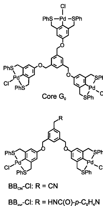
Scheme 1. Representative building blocks that have been employed to assemble metallodendrimers, see refs. [6–8]
