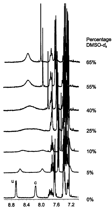
Figure 2. 1 H NMR spectra (298 K) of the titration of [D 6 ]DMSO to a CDCl 3 solution of the pyridine complex of the SCS Pd II pincer system containing an excess of 1 equiv. pyridine; the designations u and c correspond to the pyridine \alpha -proton signals of uncoordinated and coordinated pyridine, respectively
