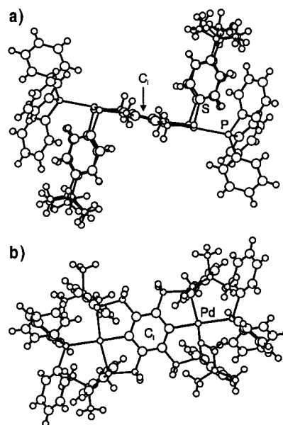
Figure 5. Structure of 3\cdot(\text{PPh}_3)_2 ; a) side view, b) top view
