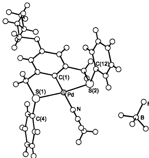
Figure 1. Structure of the acetonitrile complex 1
