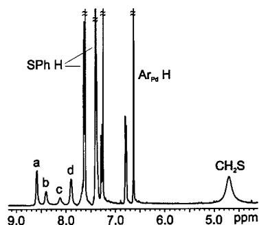
Figure 3. Part of the ^1\text{H} NMR spectrum ( \text{CDCl}_3 , 298 K) for a competition experiment between pyridine and 4-methoxypyridine. The designated signals correspond to the pyridine \alpha -proton signals of: a) free pyridine, b) free 4-methoxypyridine, c) bound pyridine, d) bound 4-methoxypyridine
