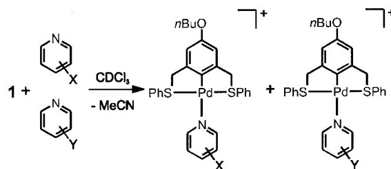
Scheme 3. Competition experiments between substituted pyridines
