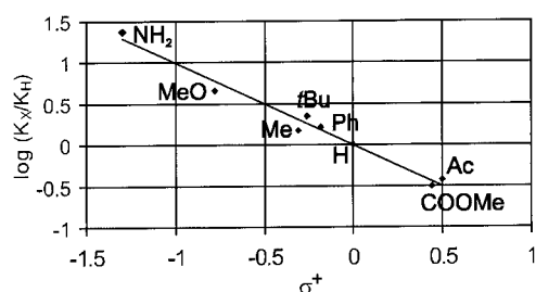
Figure 4. Hammett plot of the stability of 4-substituted pyridine complexes with the SCS \text{Pd}^{\text{II}} pincer system against the Brown-Okamoto \sigma^+ substituent constant
